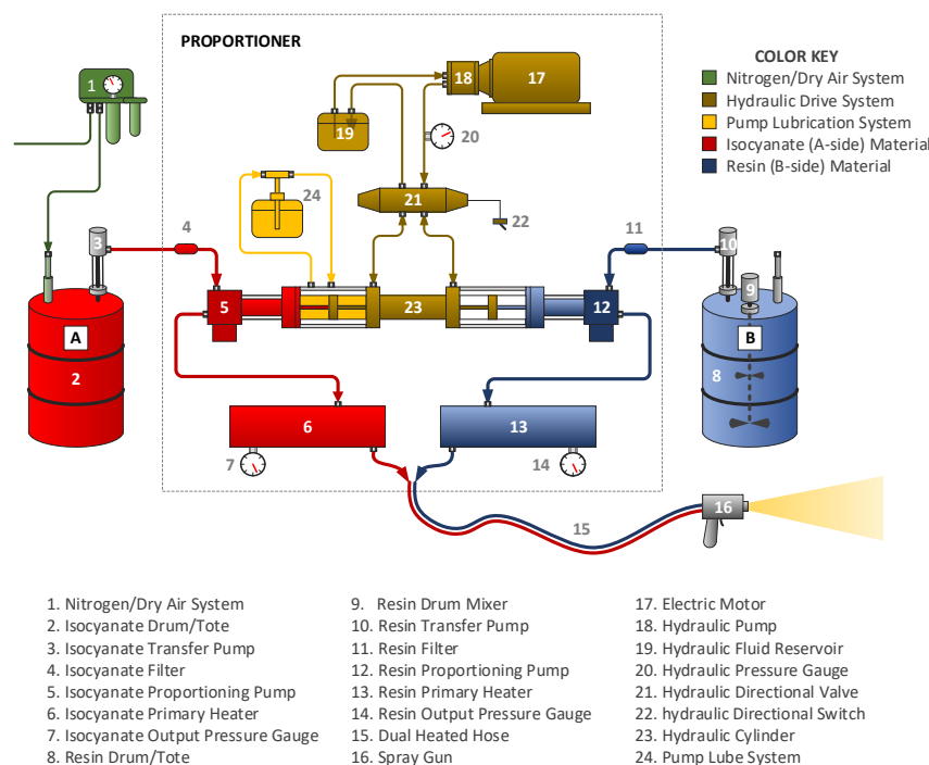
Figure 3. Schematic of a High-Pressure SPF system
